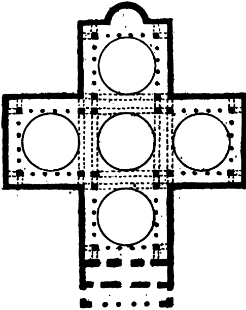
FIG. 27. Approximate plan of the church of the Holy Apostles, Constantinople.
